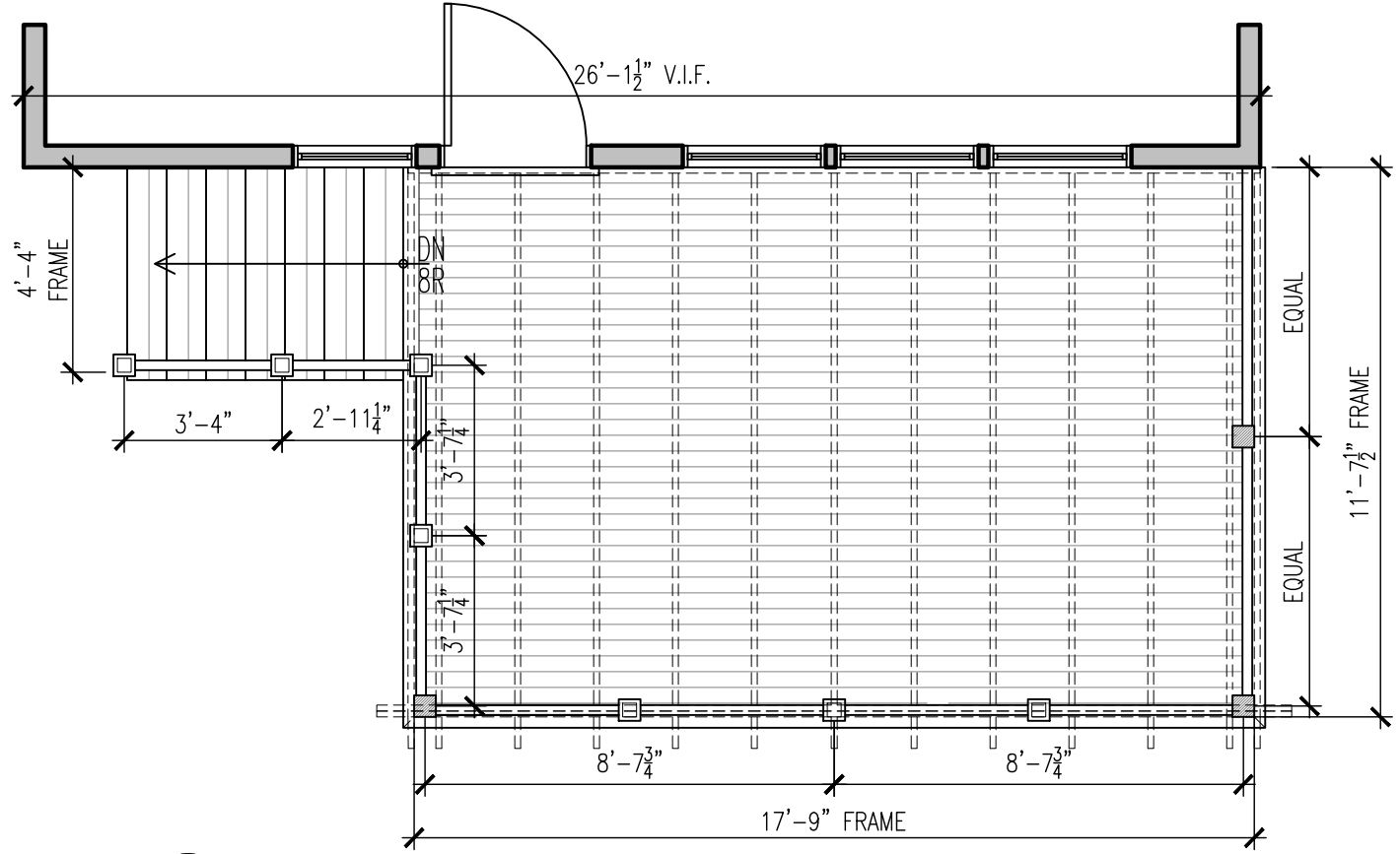
1 DECK PLAN 1/4"=1'-0"
